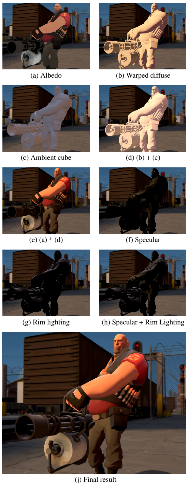
Figure 6: Individual character and model shading terms
